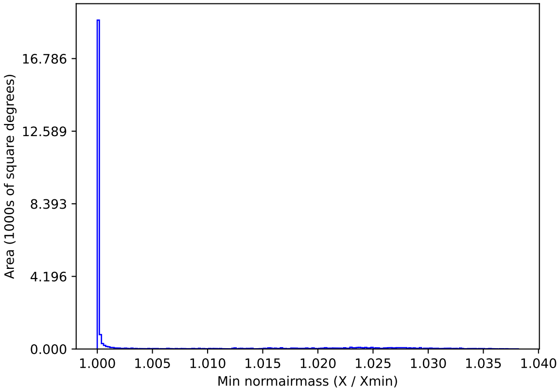
ddf_loaded_half_fl15_v3.4_10yrs All sky r band: Min normairmass
