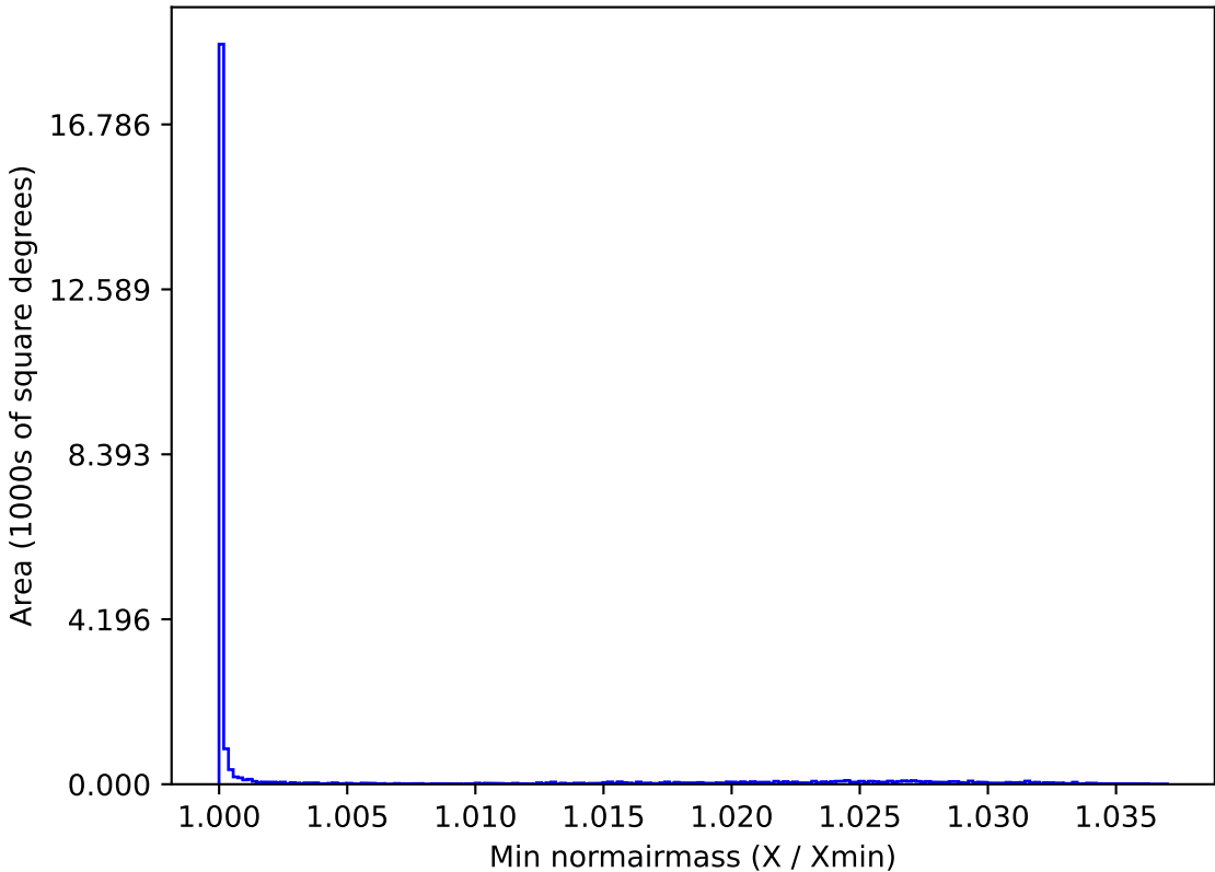
ddf_loaded_half_fl15_v3.4_10yrs All sky i band: Min normairmass
