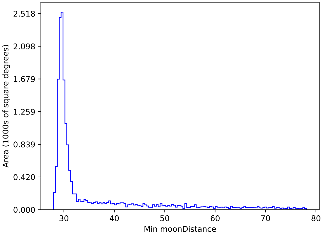
ddf_loaded_half_fl15_v3.4_10yrs WFD z band: Min moonDistance
