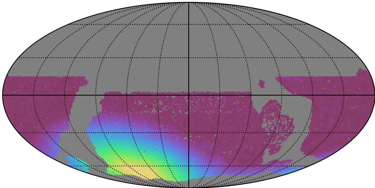
ddf_loaded_half_fl15_v3.4_10yrs WFD y band: Min moonDistance
