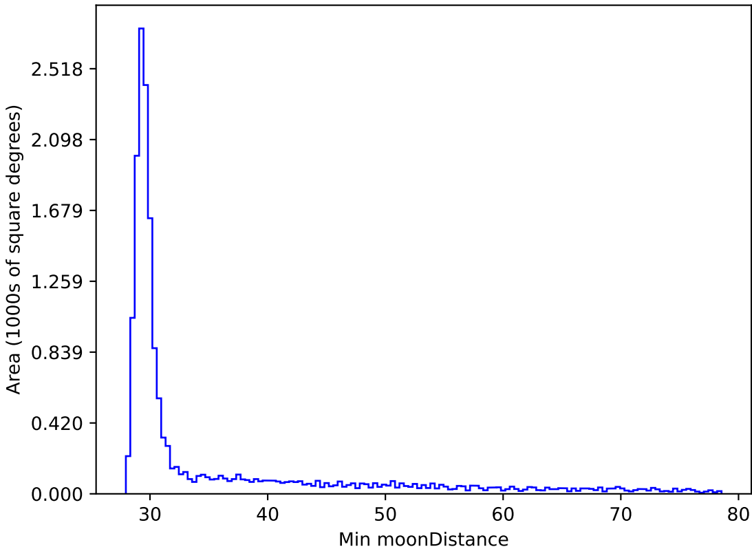
ddf_loaded_half_fl15_v3.4_10yrs WFD y band: Min moonDistance
