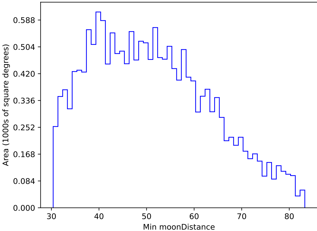
ddf_loaded_half_fl15_v3.4_10yrs WFD u band: Min moonDistance
