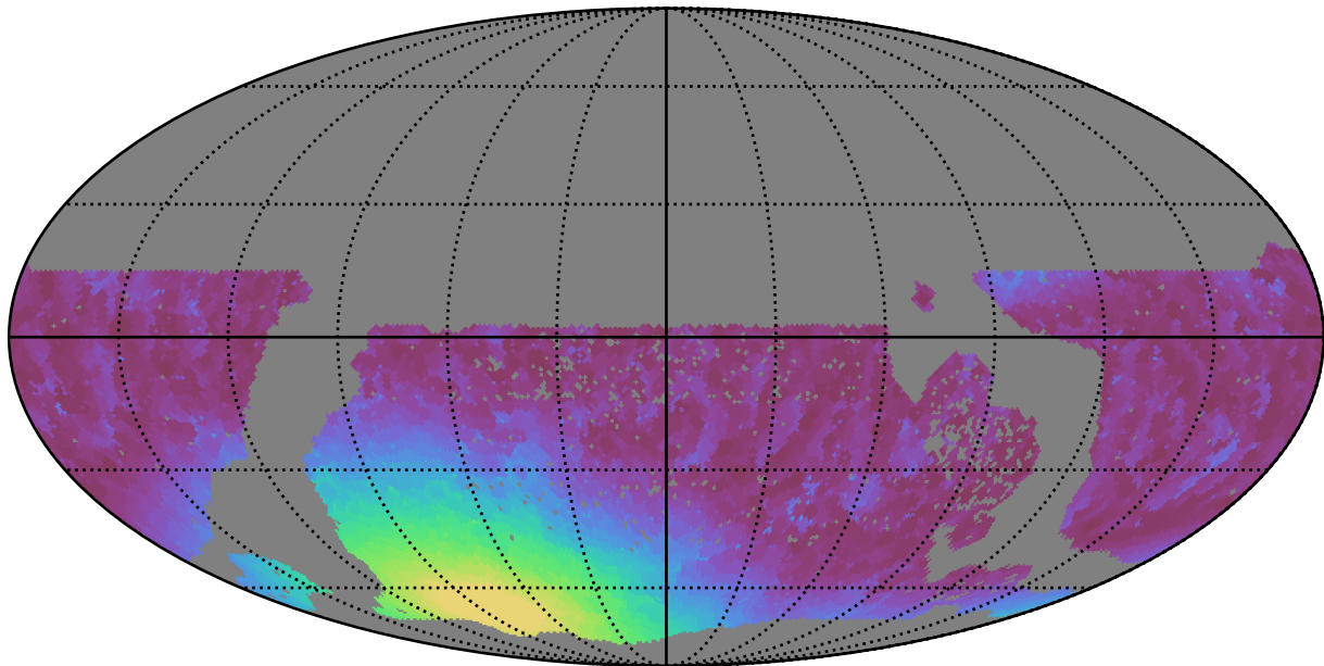
ddf_loaded_half_fl15_v3.4_10yrs WFD r band: Min moonDistance
