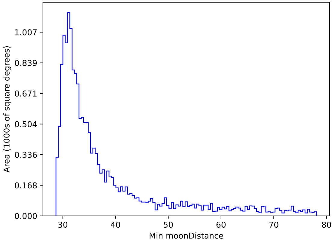
ddf_loaded_half_fl15_v3.4_10yrs WFD r band: Min moonDistance
