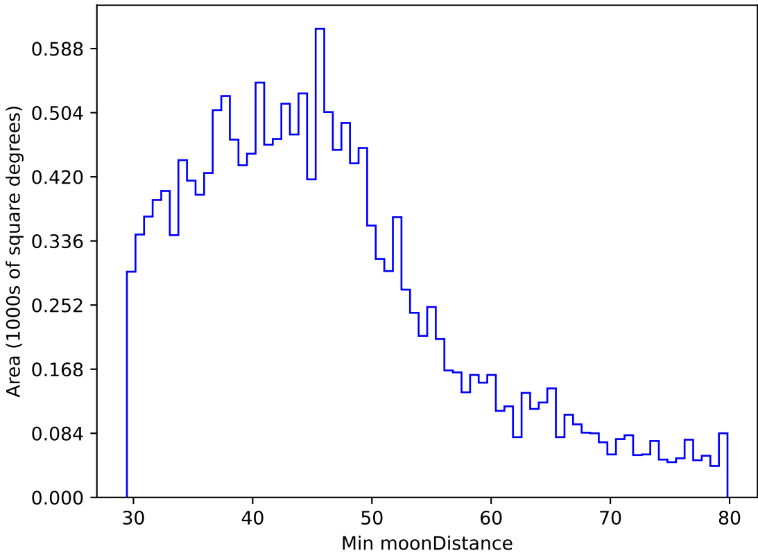
ddf_loaded_half_fl15_v3.4_10yrs WFD g band: Min moonDistance
