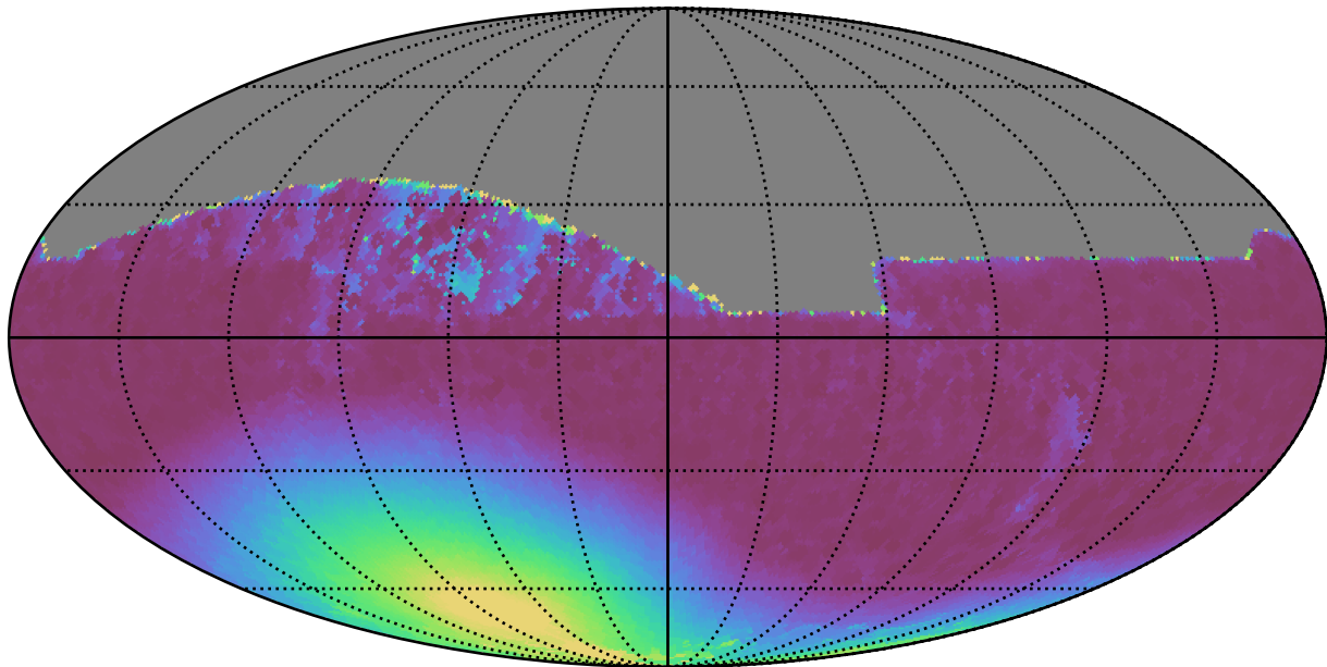
ddf_loaded_half_fl15_v3.4_10yrs All sky z band: Min moonDistance
