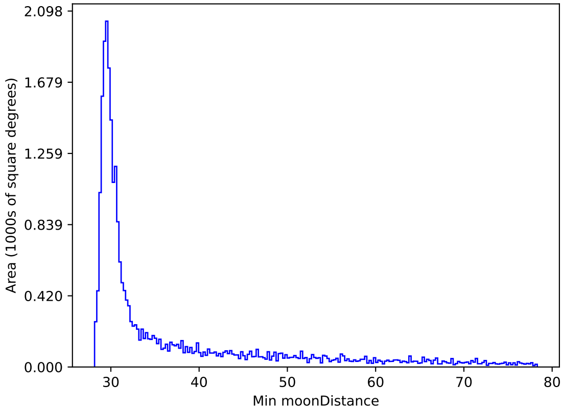
ddf_loaded_half_fl15_v3.4_10yrs All sky z band: Min moonDistance
