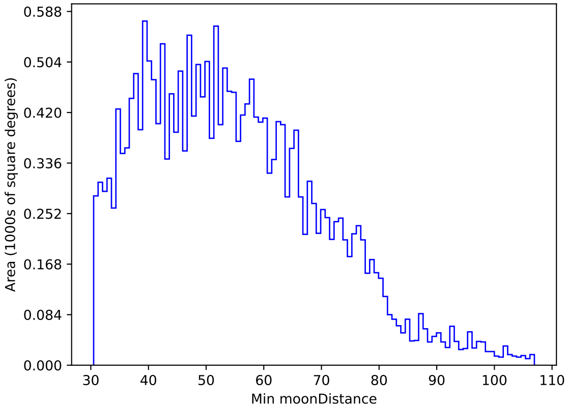
ddf_loaded_half_fl15_v3.4_10yrs All sky u band: Min moonDistance
