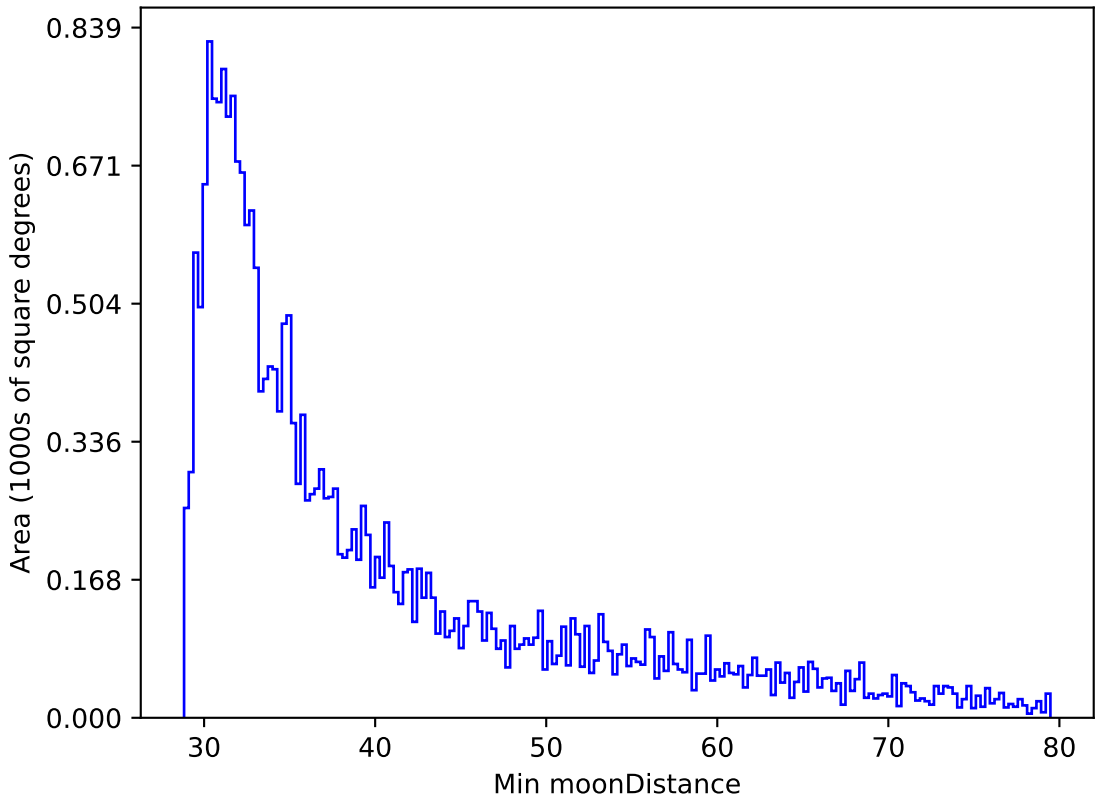
ddf_loaded_half_fl15_v3.4_10yrs All sky r band: Min moonDistance
