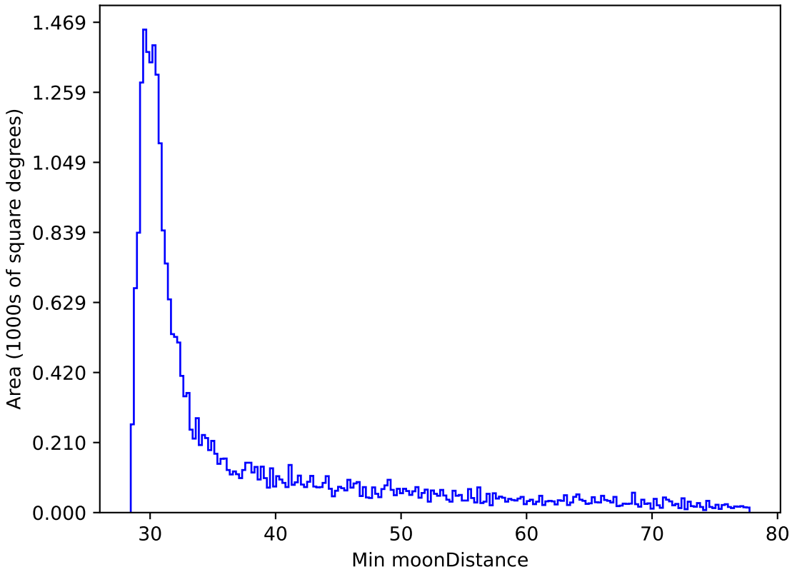
ddf_loaded_half_fl15_v3.4_10yrs All sky i band: Min moonDistance
