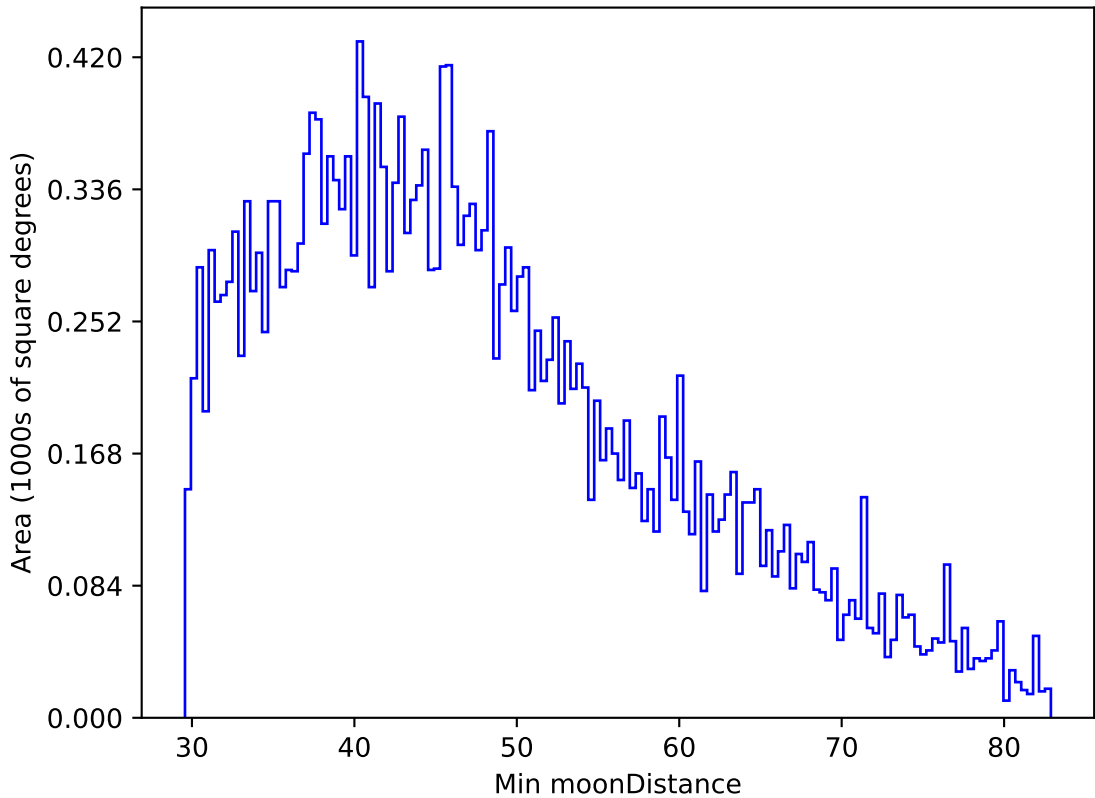
ddf_loaded_half_fl15_v3.4_10yrs All sky g band: Min moonDistance
