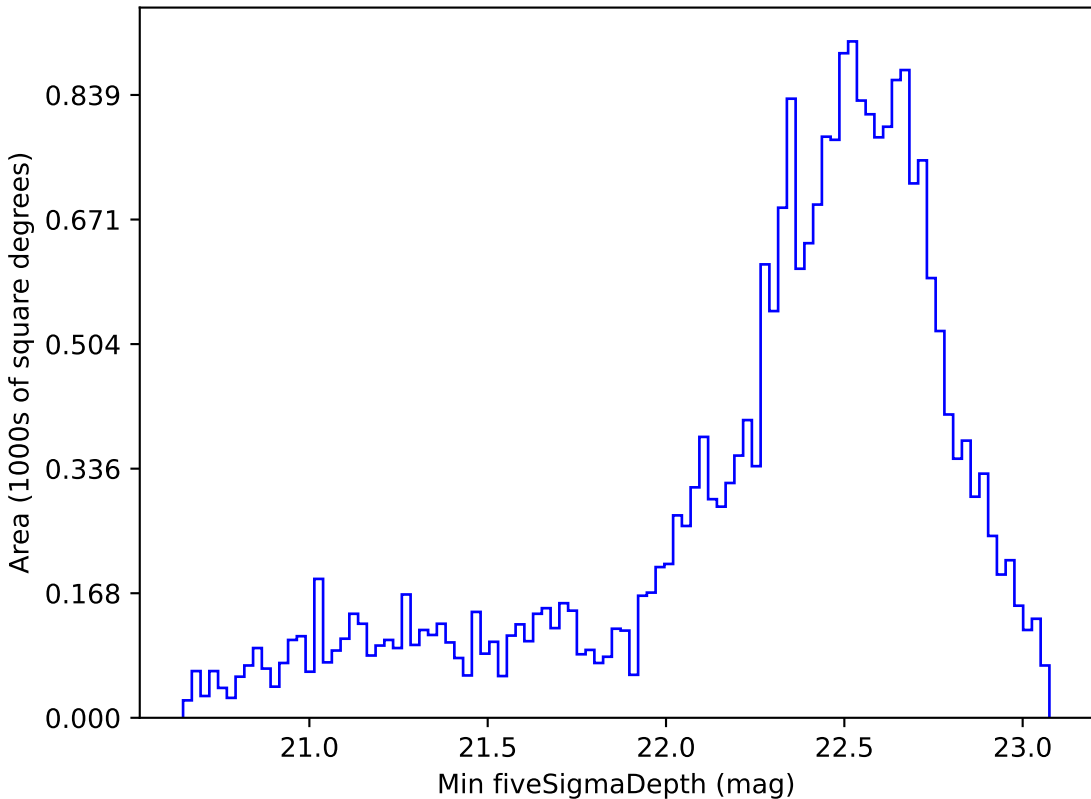
ddf_loaded_half_fl15_v3.4_10yrs Yr 1 z band: Min fiveSigmaDepth
