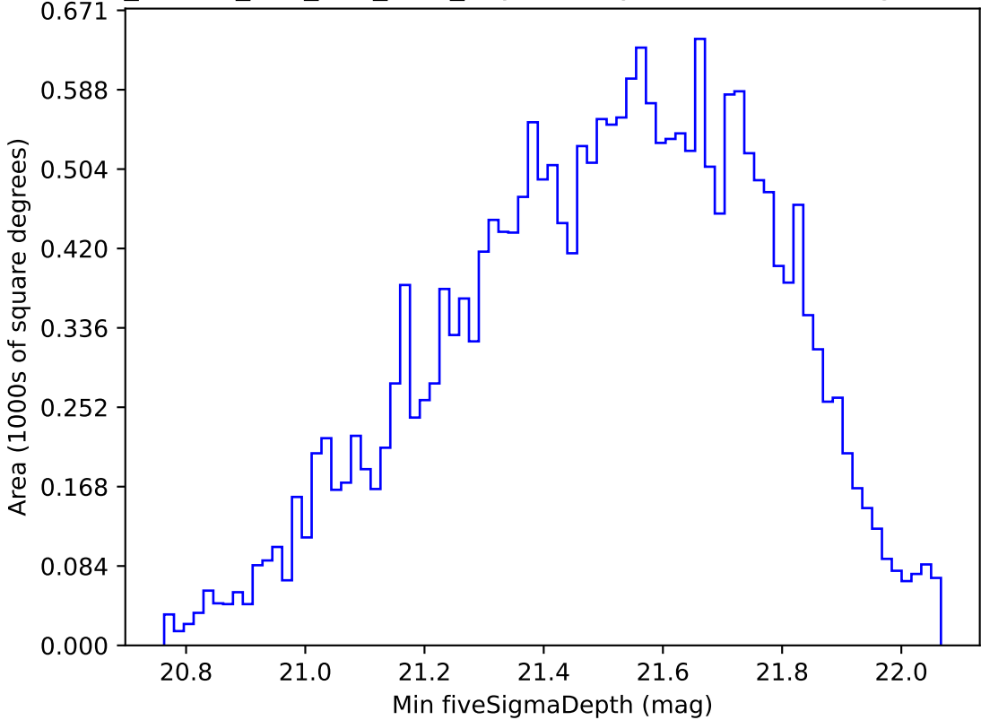
ddf_loaded_half_fl15_v3.4_10yrs Yr 1 y band: Min fiveSigmaDepth
