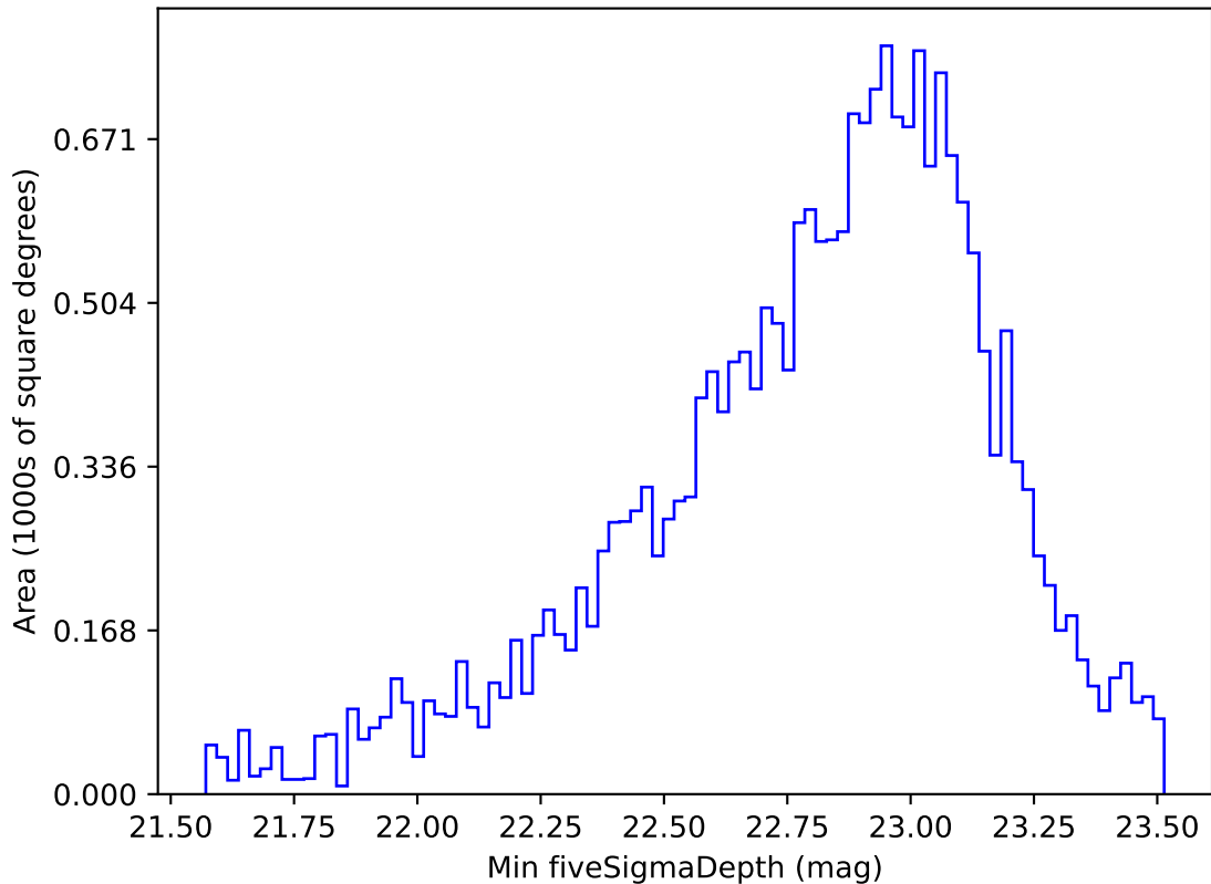
ddf_loaded_half_fl15_v3.4_10yrs Yr 1 u band: Min fiveSigmaDepth
