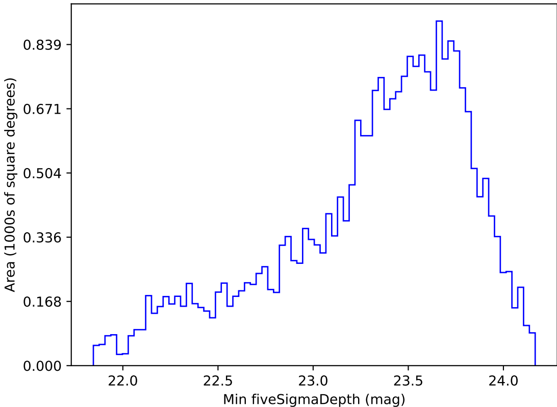
ddf_loaded_half_fl15_v3.4_10yrs Yr 1 r band: Min fiveSigmaDepth
