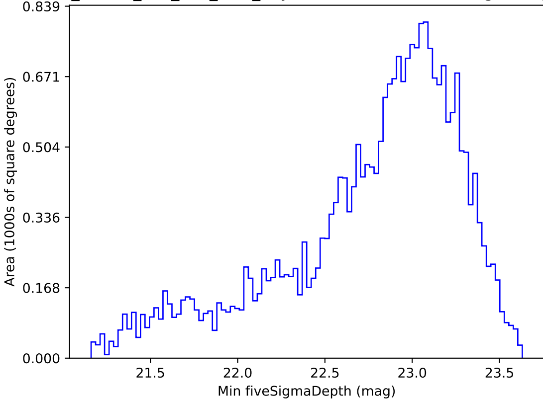
ddf_loaded_half_fl15_v3.4_10yrs Yr 1 i band: Min fiveSigmaDepth
