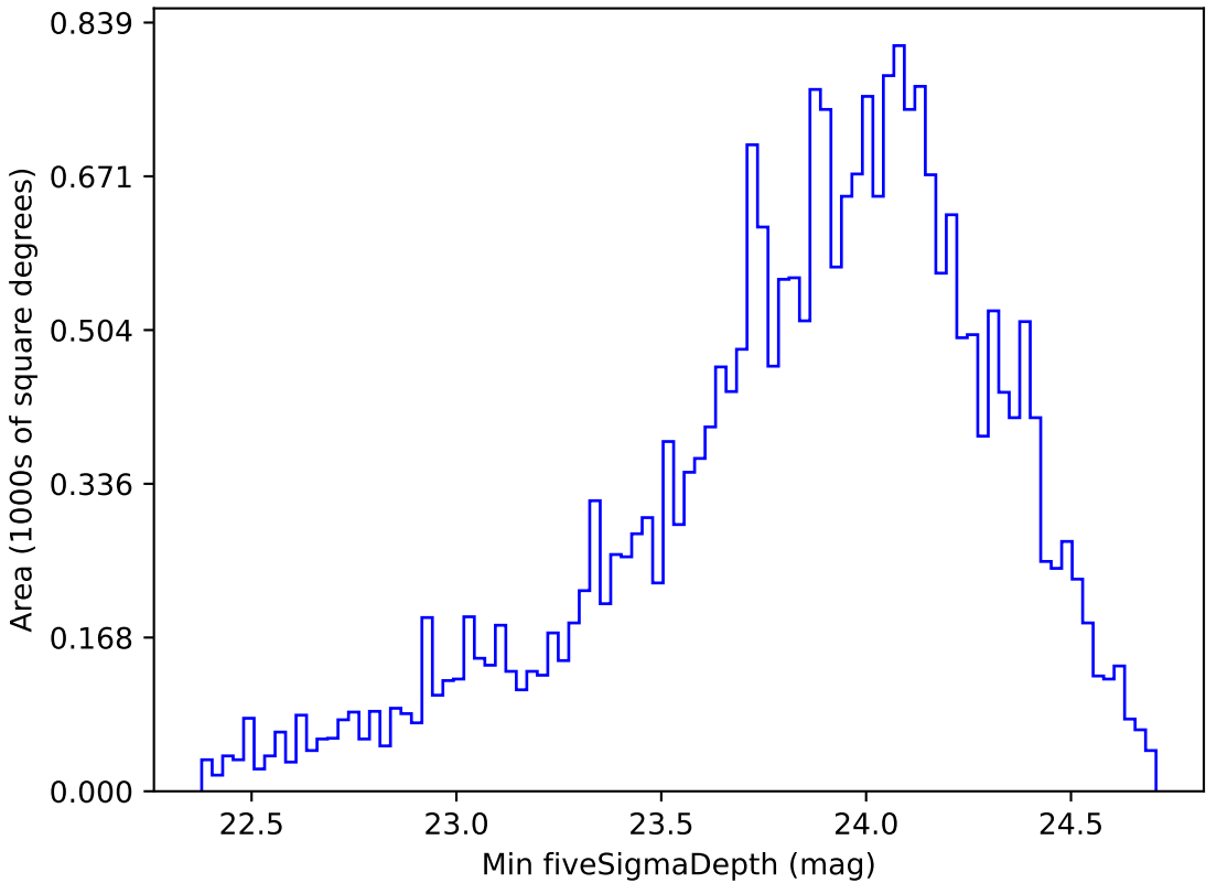
ddf_loaded_half_fl15_v3.4_10yrs Yr 1 g band: Min fiveSigmaDepth
