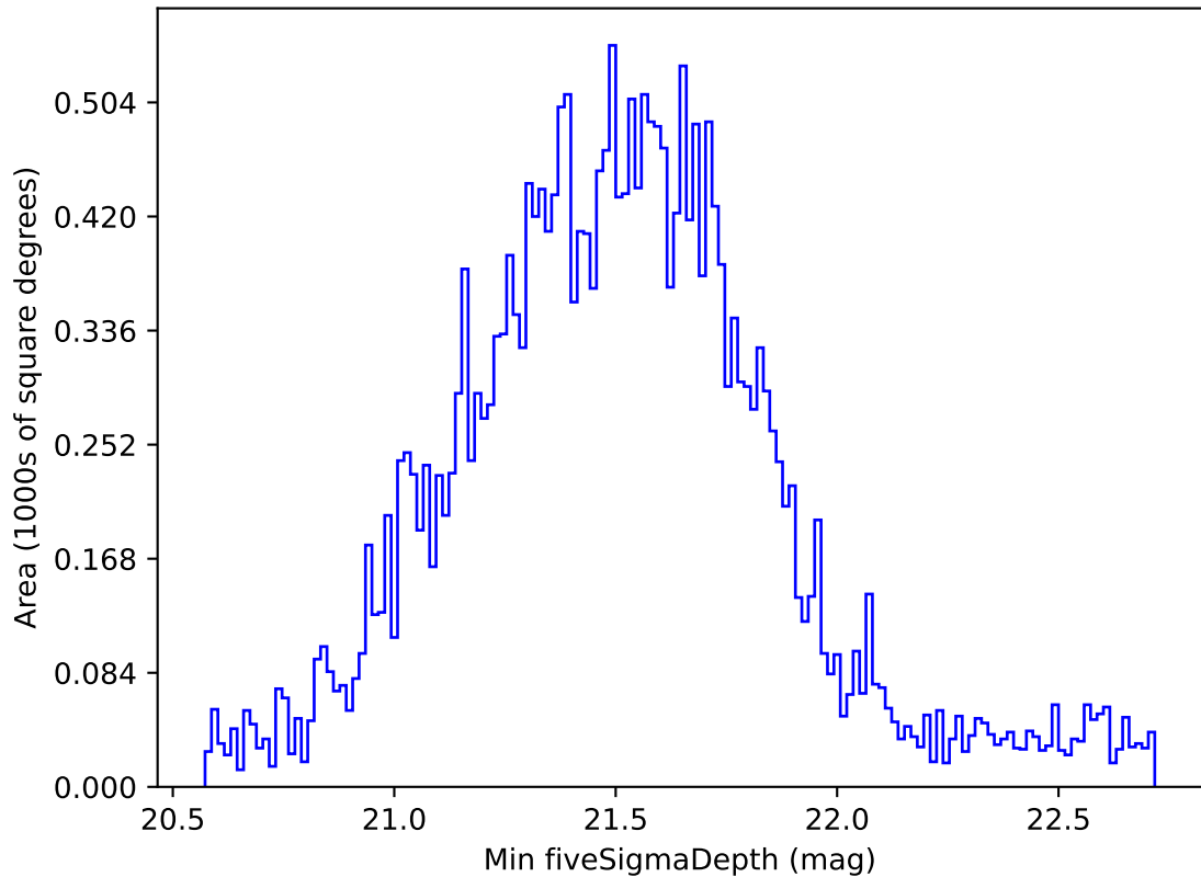
ddf_loaded_half_fl15_v3.4_10yrs Yr 1 all bands: Min fiveSigmaDepth
