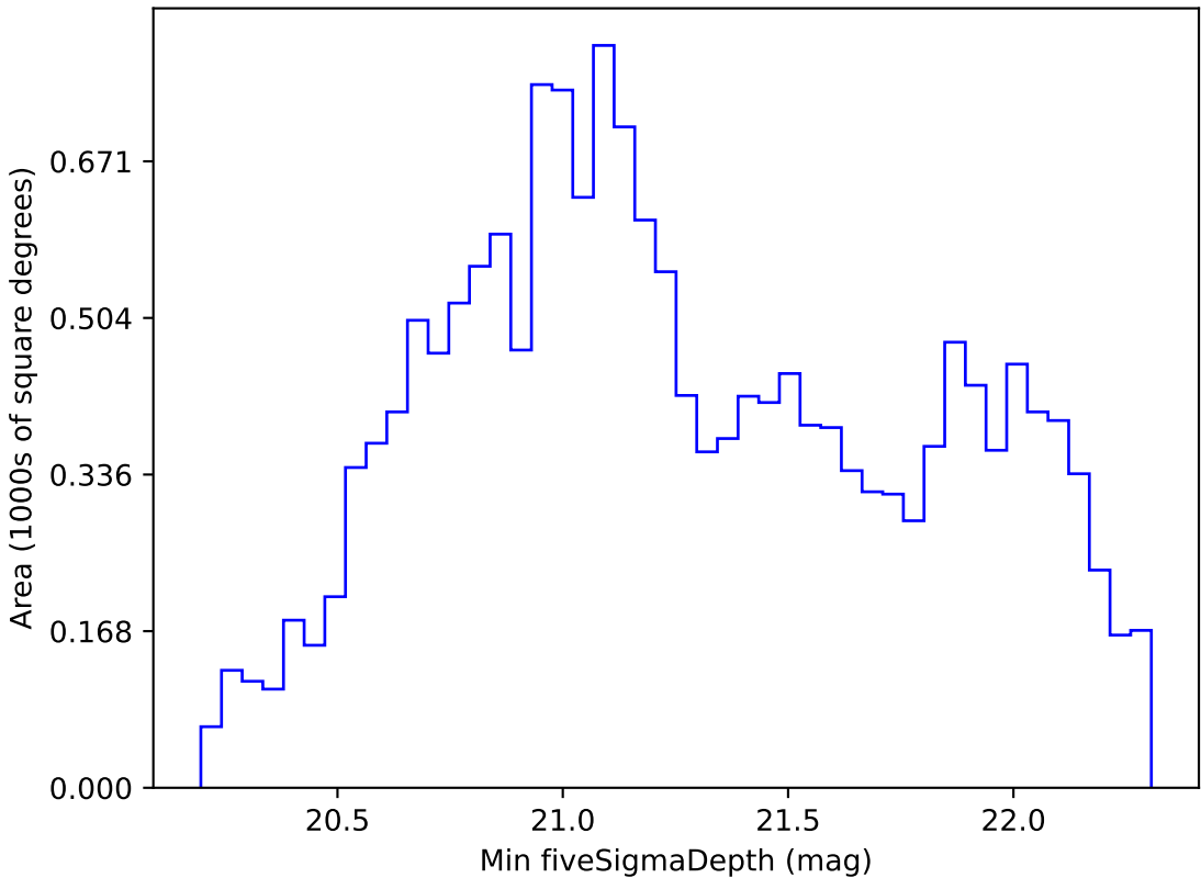
ddf_loaded_half_fl15_v3.4_10yrs WFD z band: Min fiveSigmaDepth
