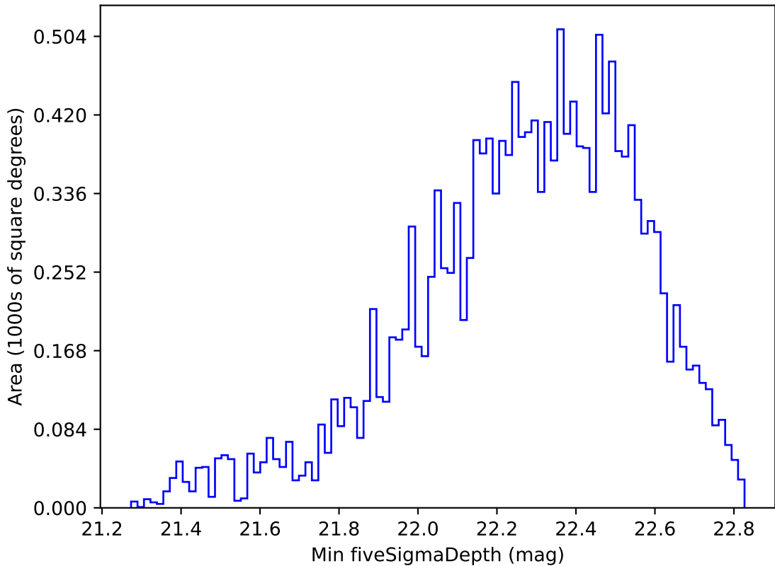
ddf_loaded_half_fl15_v3.4_10yrs WFD u band: Min fiveSigmaDepth
