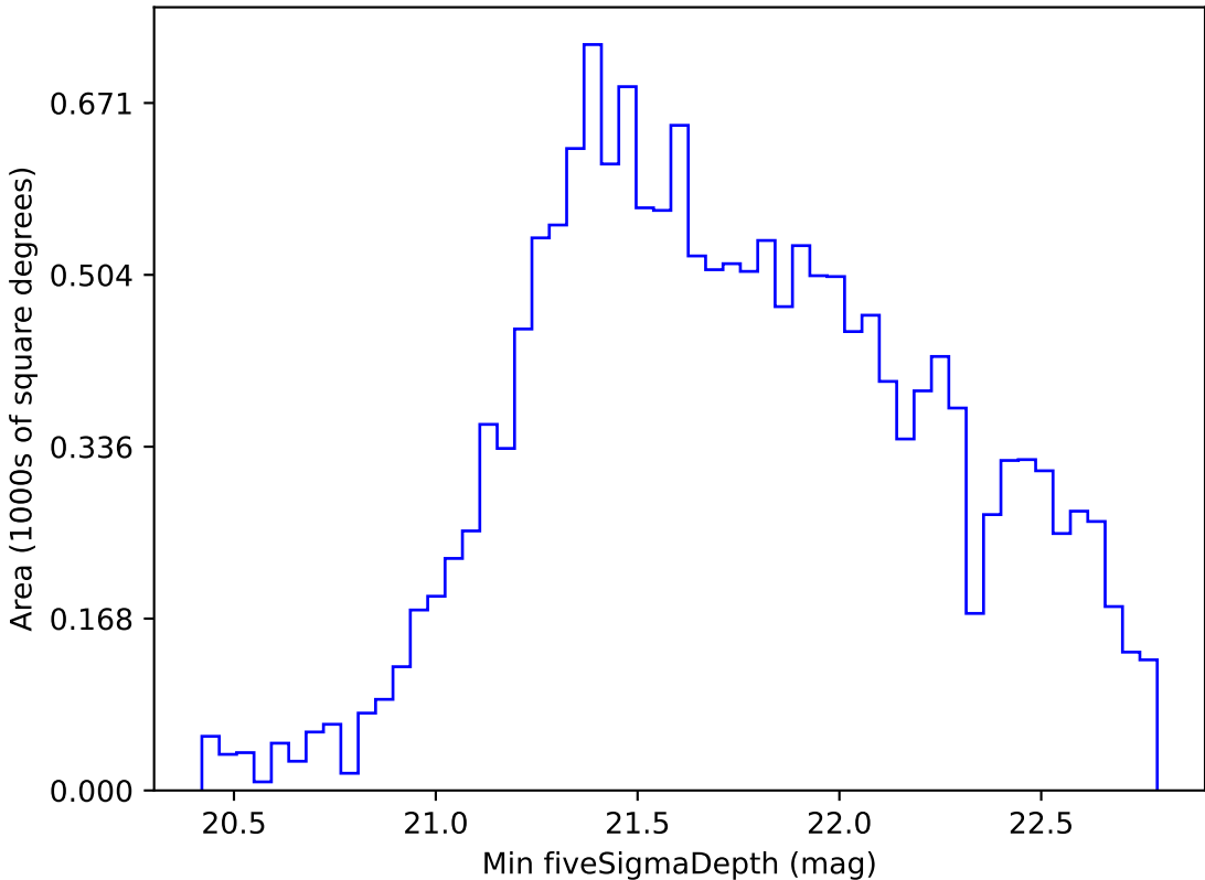
ddf_loaded_half_fl15_v3.4_10yrs WFD i band: Min fiveSigmaDepth
