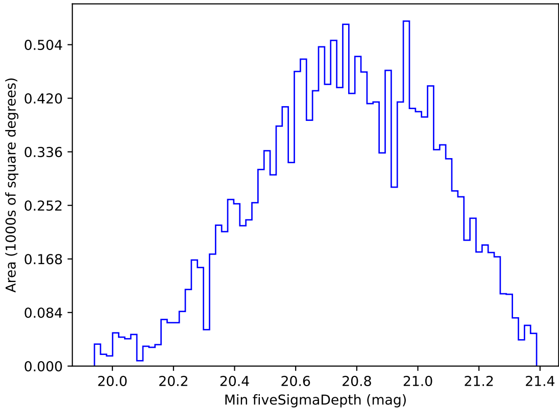
ddf_loaded_half_fl15_v3.4_10yrs WFD all bands: Min fiveSigmaDepth
