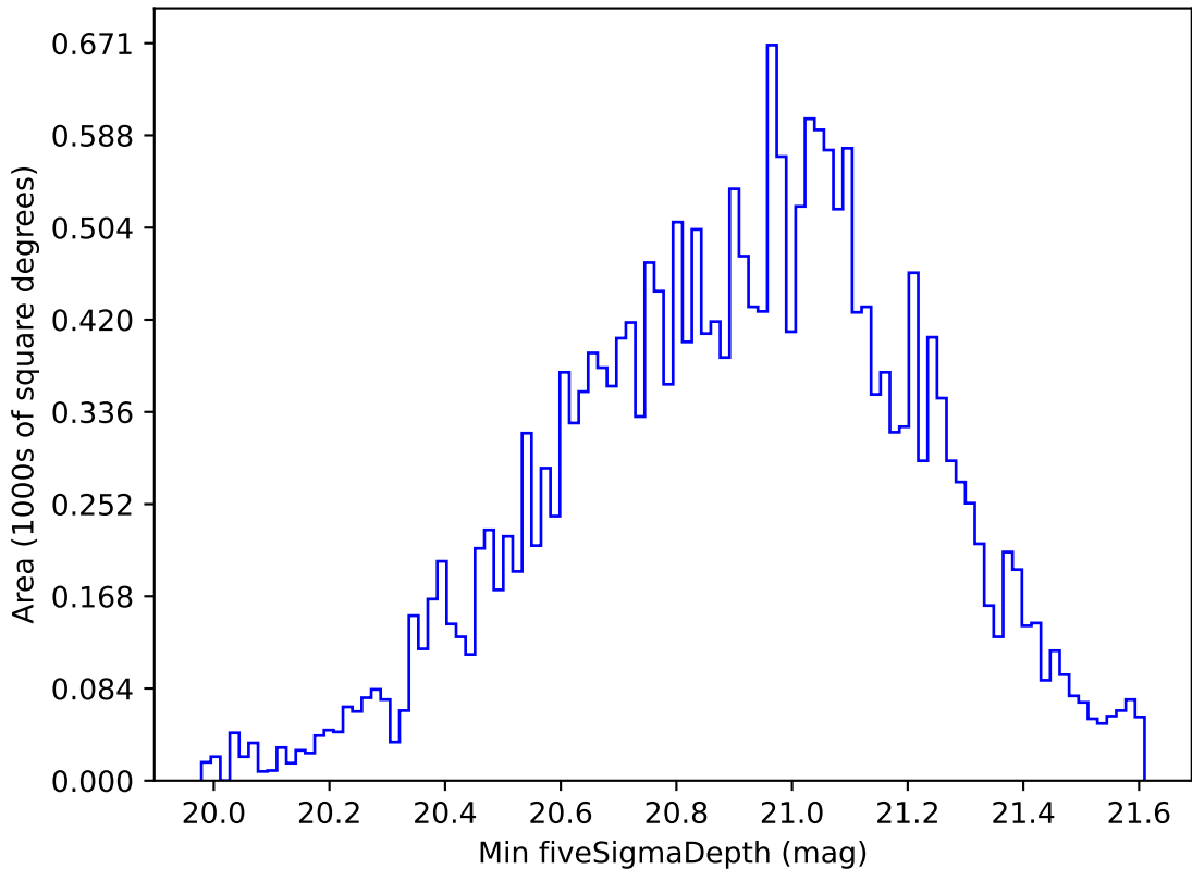
ddf_loaded_half_fl15_v3.4_10yrs All sky y band: Min fiveSigmaDepth
