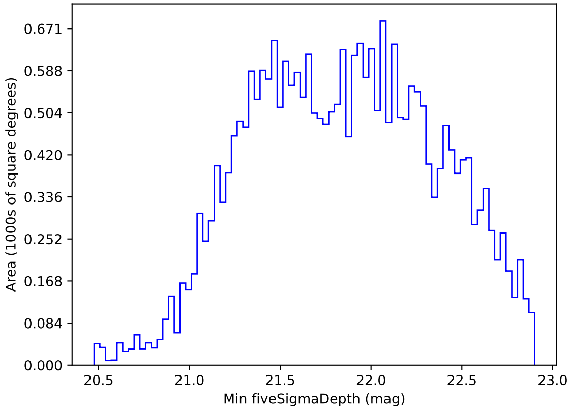
ddf_loaded_half_fl15_v3.4_10yrs All sky i band: Min fiveSigmaDepth
