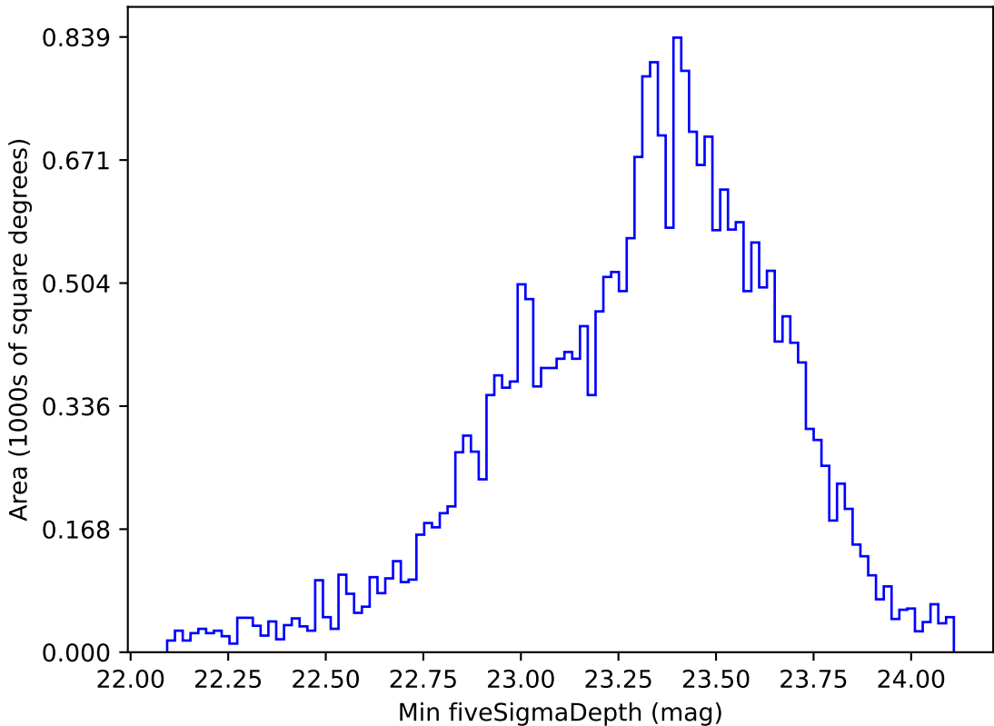
ddf_loaded_half_fl15_v3.4_10yrs All sky g band: Min fiveSigmaDepth
