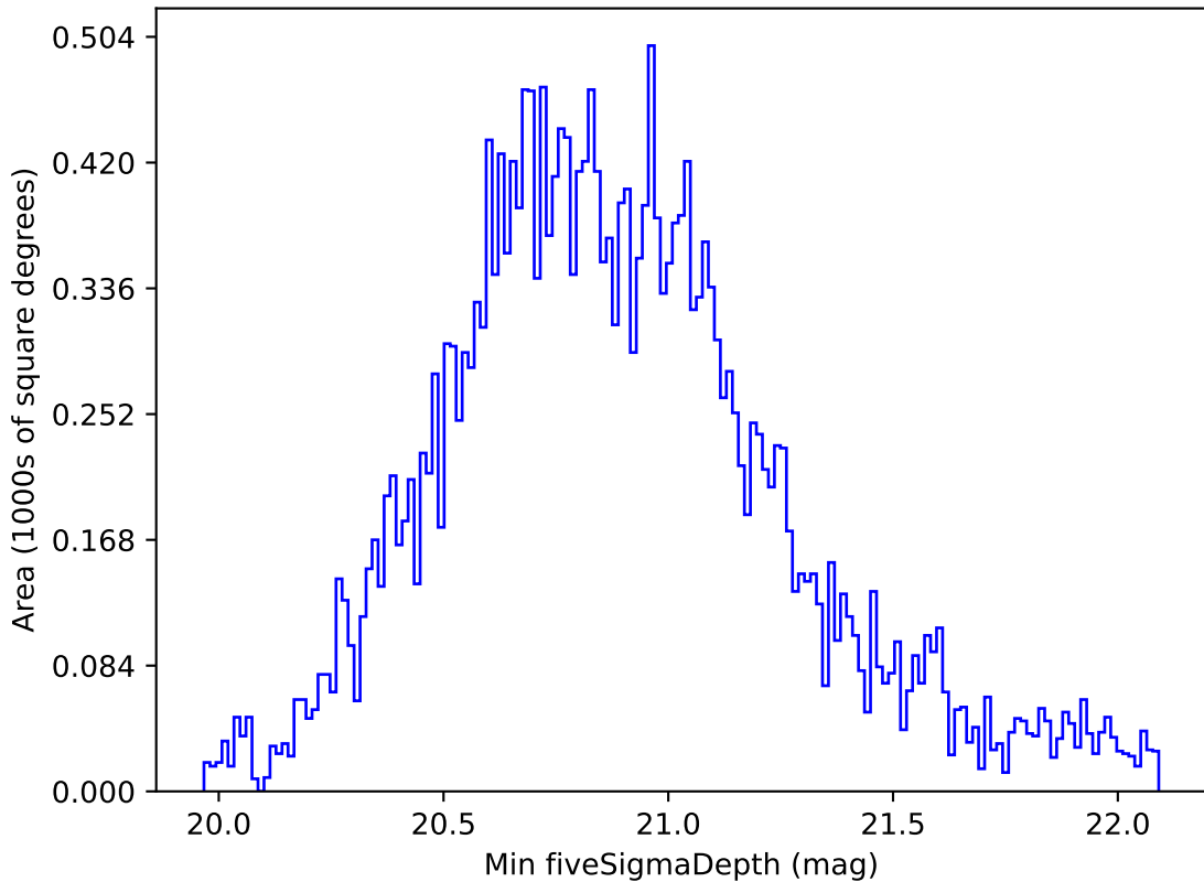
ddf_loaded_half_fl15_v3.4_10yrs All sky all bands: Min fiveSigmaDepth
