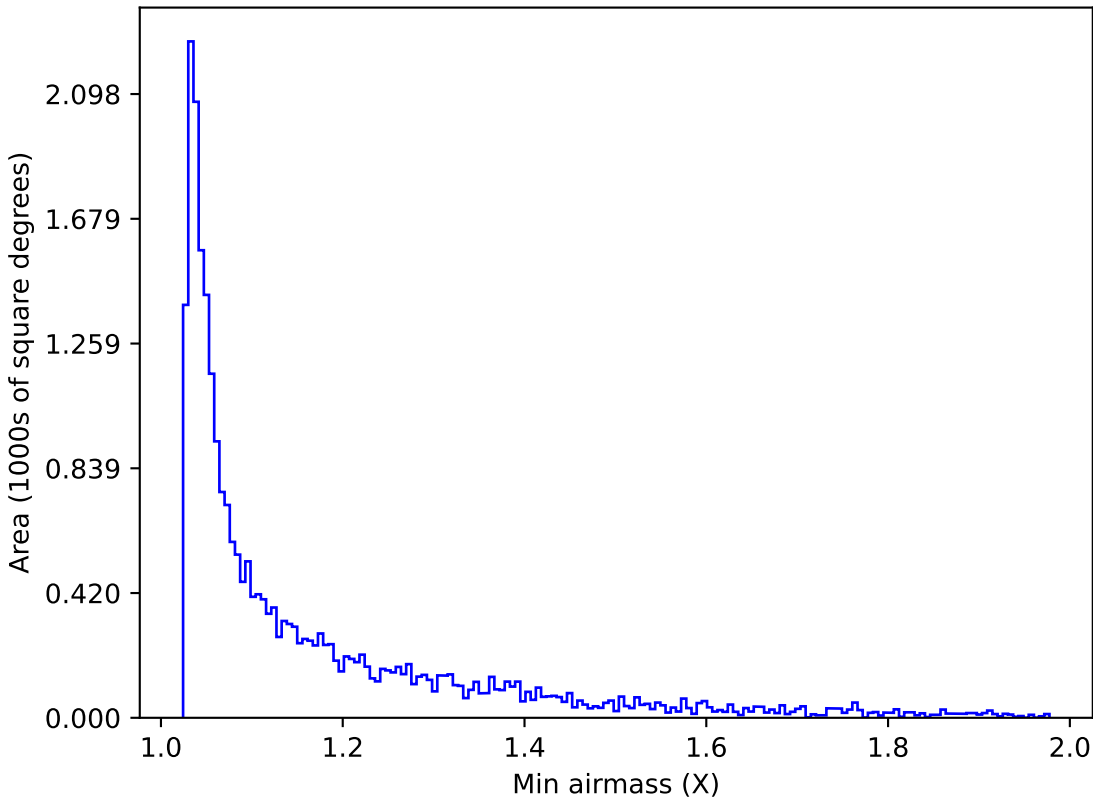
ddf_loaded_half_fl15_v3.4_10yrs Yr 1 z band: Min airmass
