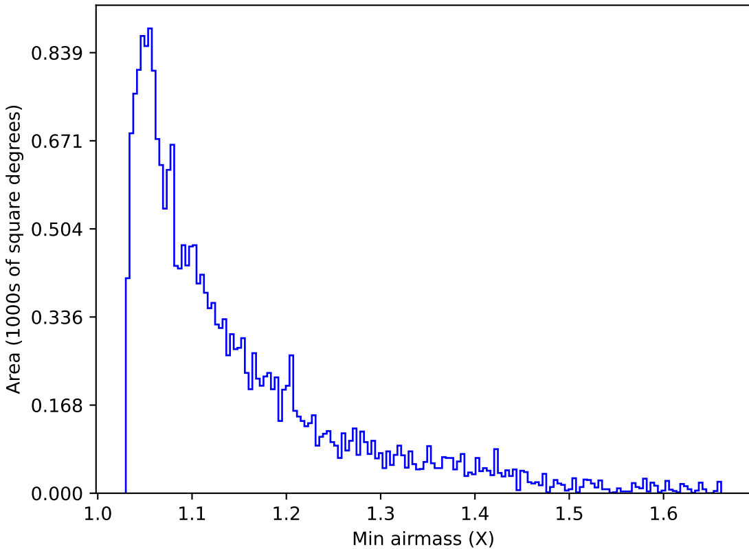
ddf_loaded_half_fl15_v3.4_10yrs Yr 1 u band: Min airmass
