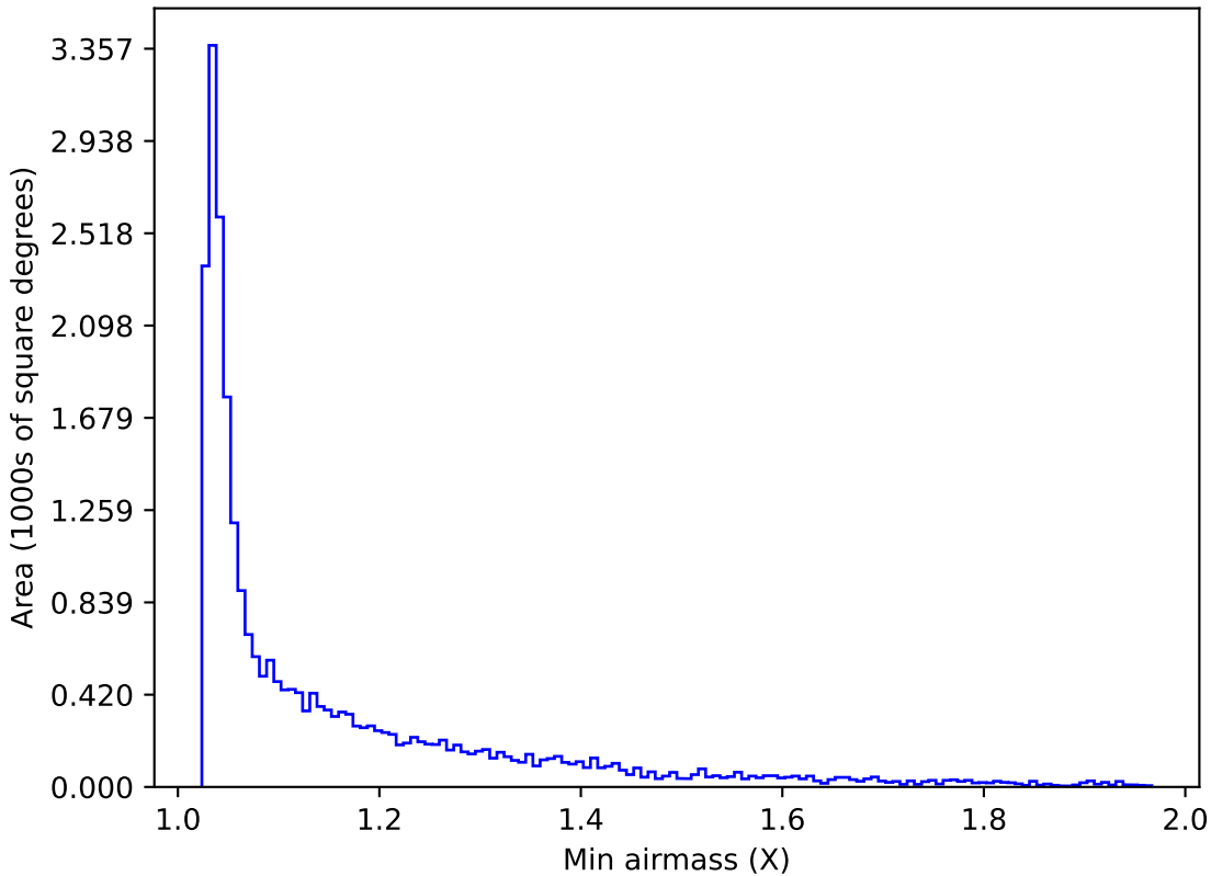
ddf_loaded_half_fl15_v3.4_10yrs Yr 1 i band: Min airmass
