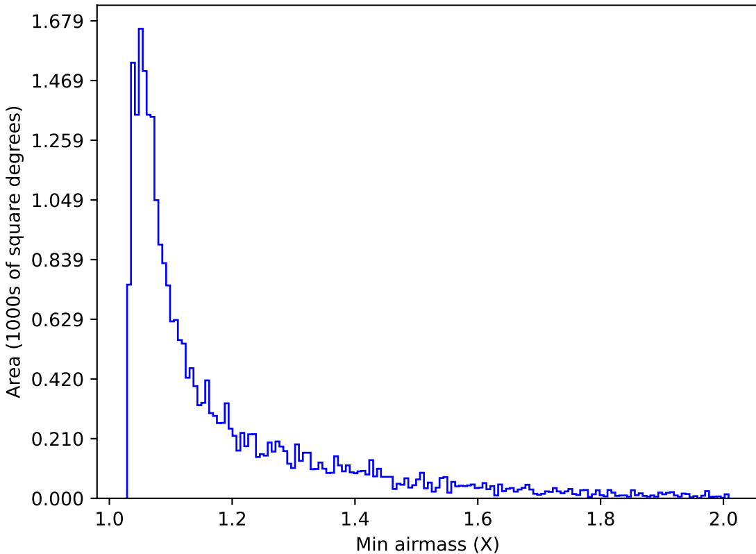
ddf_loaded_half_fl15_v3.4_10yrs Yr 1 g band: Min airmass
