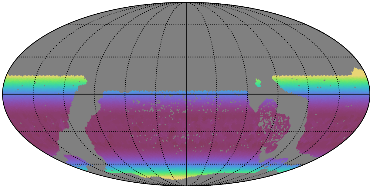
ddf_loaded_half_fl15_v3.4_10yrs WFD z band: Min airmass
