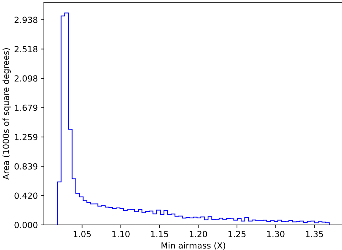
ddf_loaded_half_fl15_v3.4_10yrs WFD z band: Min airmass
