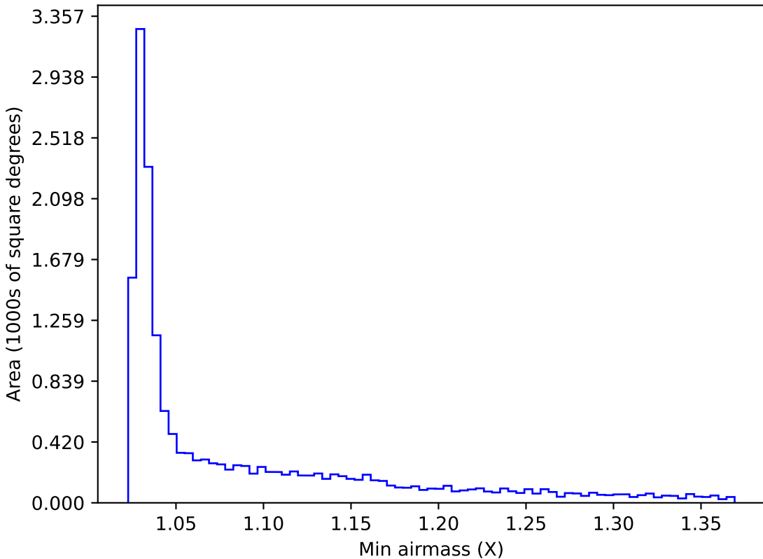
ddf_loaded_half_fl15_v3.4_10yrs WFD y band: Min airmass
