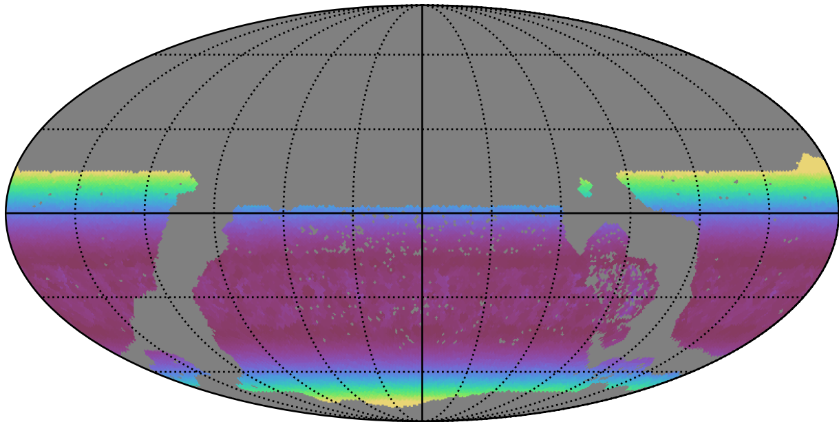
ddf_loaded_half_fl15_v3.4_10yrs WFD u band: Min airmass
