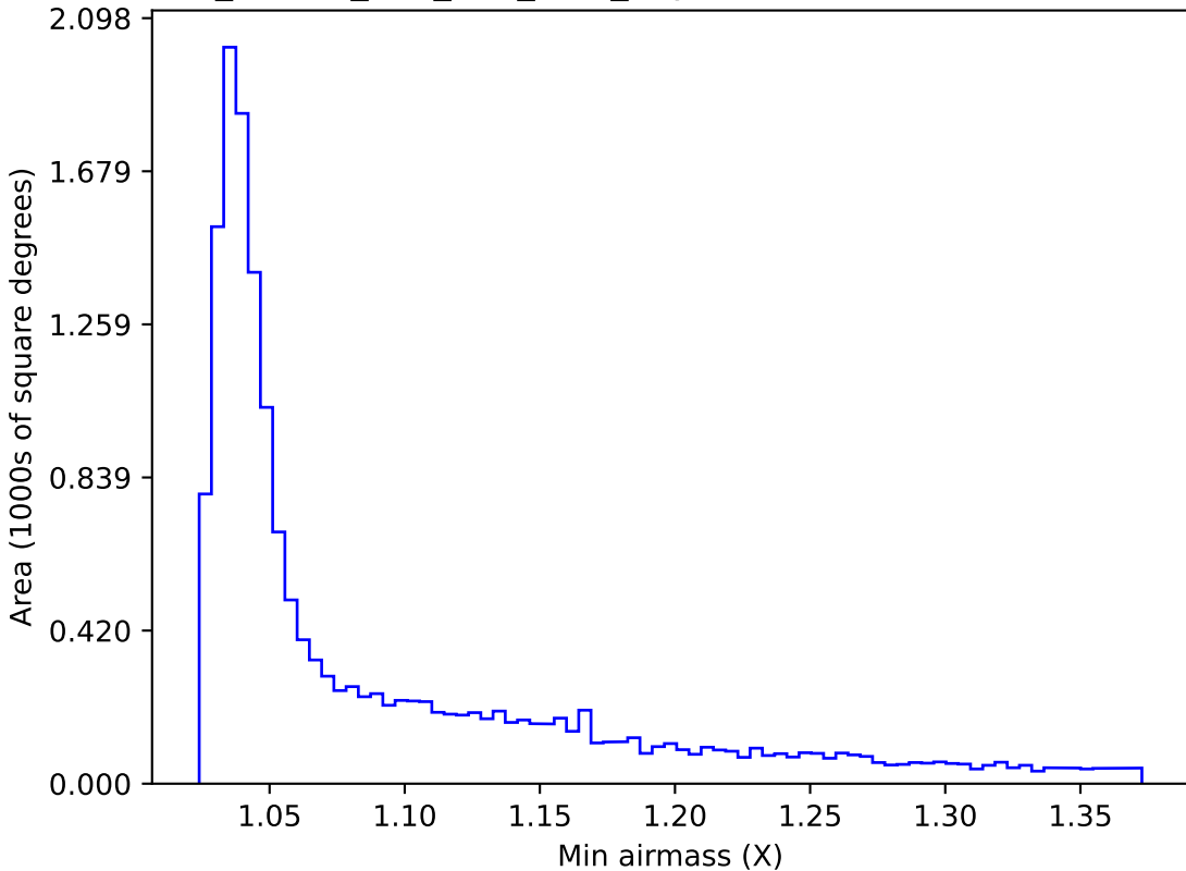
ddf_loaded_half_fl15_v3.4_10yrs WFD u band: Min airmass
