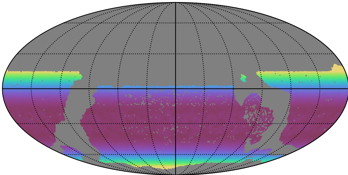
ddf_loaded_half_fl15_v3.4_10yrs WFD r band: Min airmass
