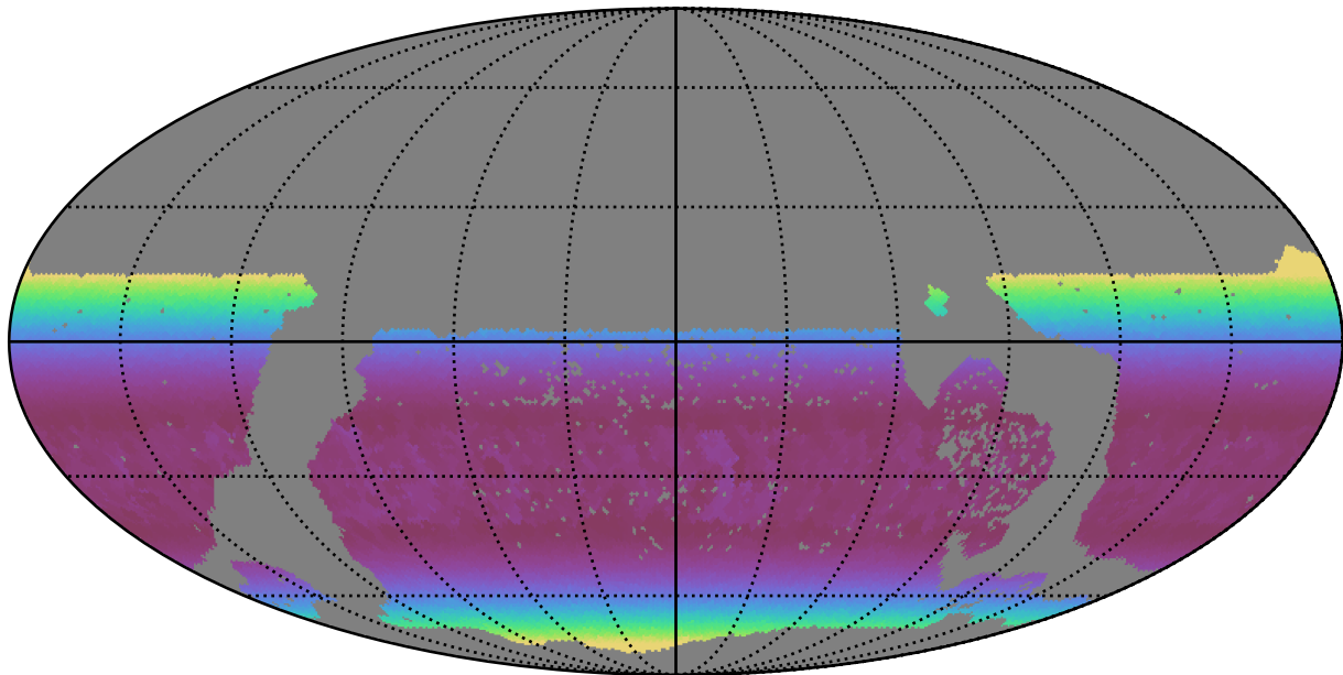
ddf_loaded_half_fl15_v3.4_10yrs WFD g band: Min airmass
