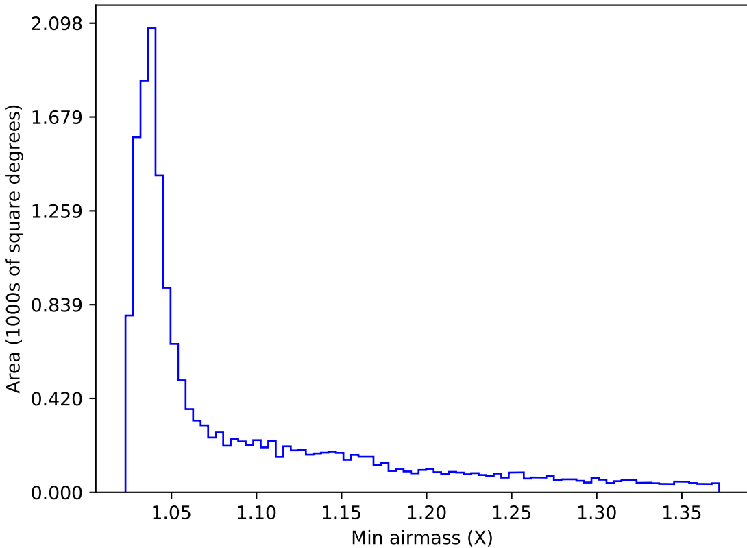
ddf_loaded_half_fl15_v3.4_10yrs WFD g band: Min airmass
