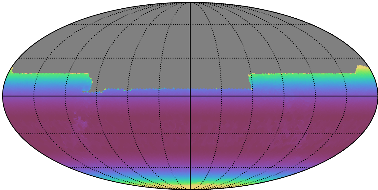
ddf_loaded_half_fl15_v3.4_10yrs All sky y band: Min airmass
