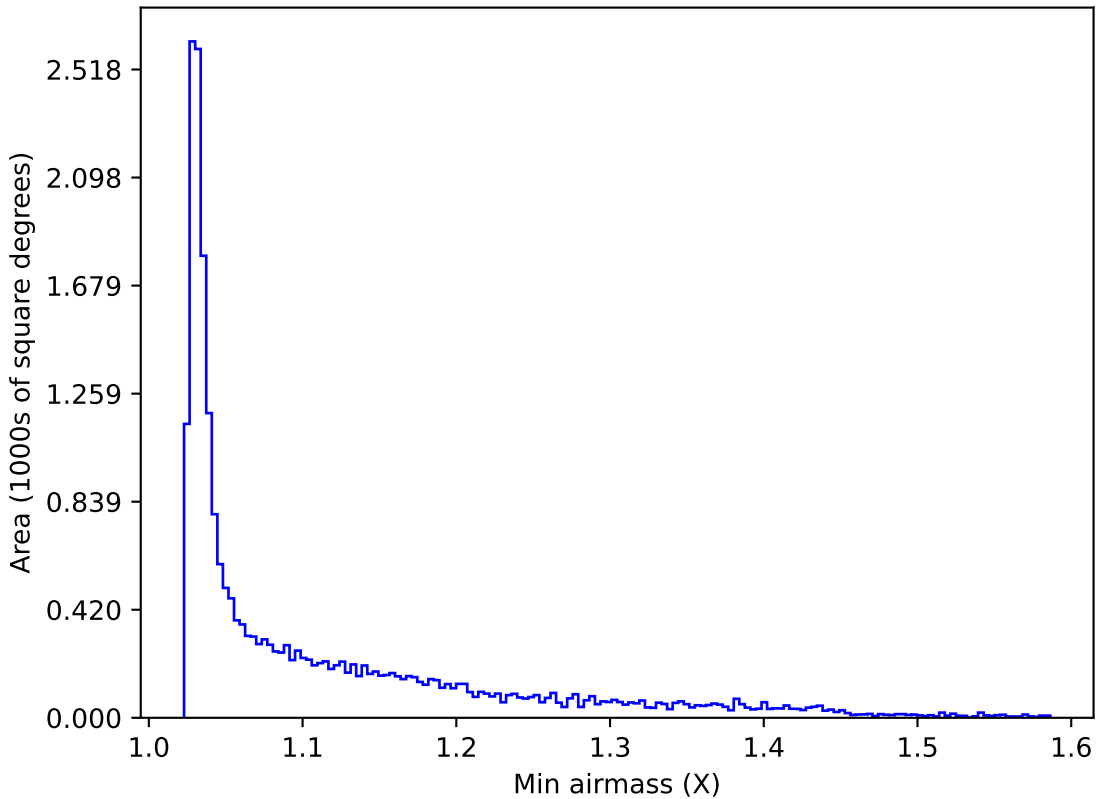
ddf_loaded_half_fl15_v3.4_10yrs All sky y band: Min airmass
