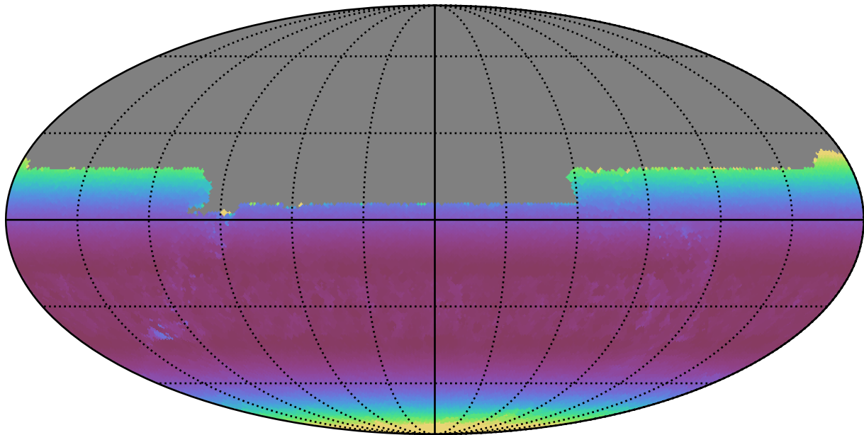
ddf_loaded_half_fl15_v3.4_10yrs All sky u band: Min airmass
