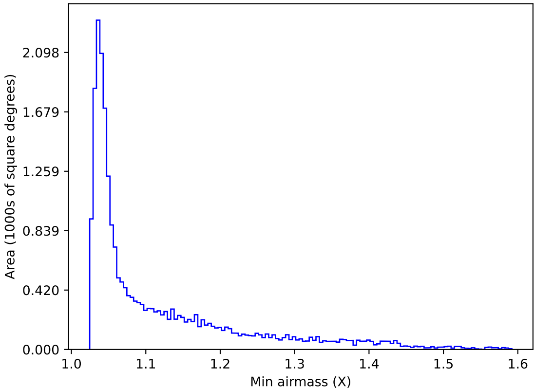
ddf_loaded_half_fl15_v3.4_10yrs All sky u band: Min airmass
