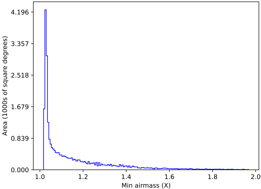
ddf_loaded_half_fl15_v3.4_10yrs All sky r band: Min airmass
