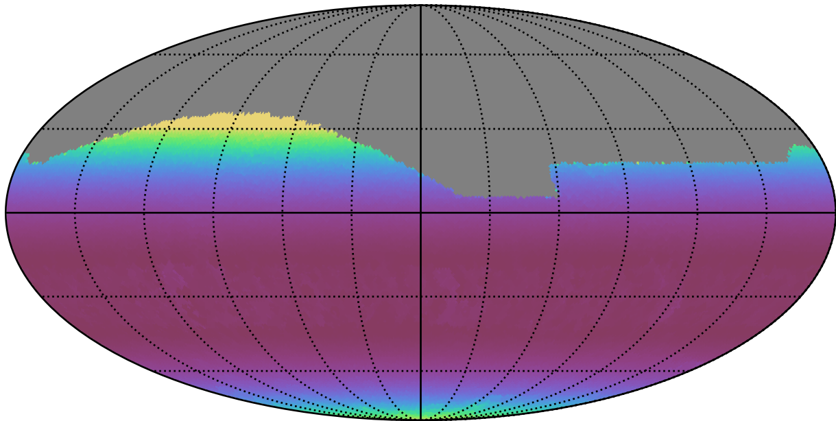
ddf_loaded_half_fl15_v3.4_10yrs All sky g band: Min airmass
