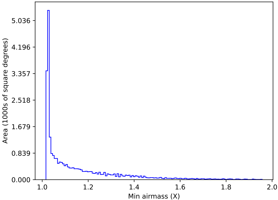
ddf_loaded_half_fl15_v3.4_10yrs All sky all bands: Min airmass
