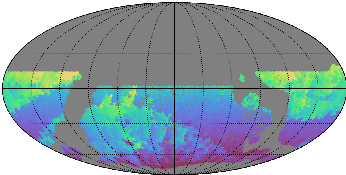
ddf_loaded_half_fl15_v3.4_10yrs WFD r band: Min HA
